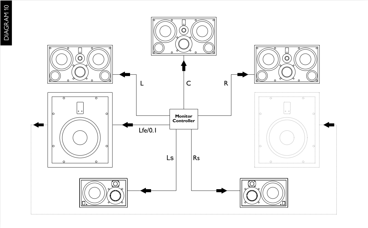
Diagram 10 – Typical Multichannel System wiring. Depending on the Monitor Controller output level and number of subwoofers, the Gain switches may need to be set to 6dB. Further subwoofers can be added to the system using the same “Daisy Chain” method shown. The system shown is an example and other configurations are available.
