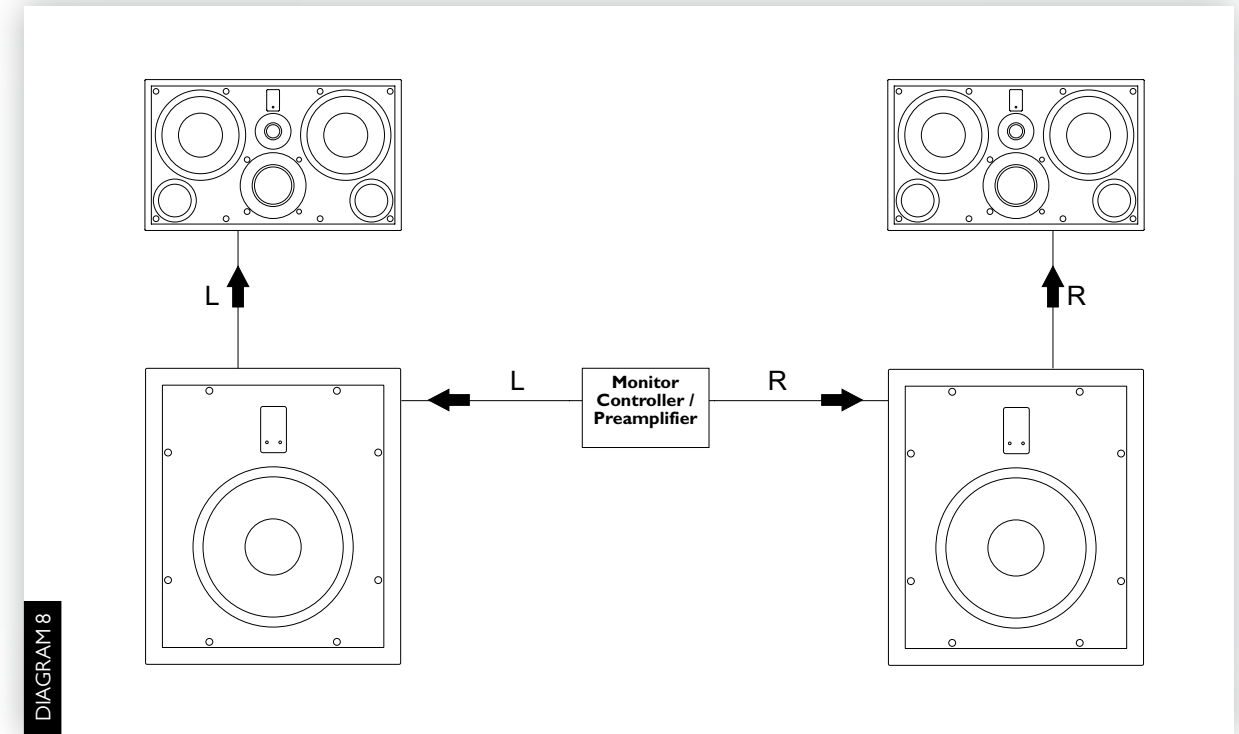
Diagram 8 – Typical Configuration – Stereo playback (Stereo Subs). A monitor controller or preamplifier output is connected to a single Input on each subwoofer. The corresponding Output of each subwoofer is connected to the Input of the main monitor on that channel. Note that it is also possible to connect the monitor controller output to both Left and Right channel Inputs on the subwoofer using a Y-Splitter cable. If connected in this way the "spare" output can be used to connect further subwoofers.
