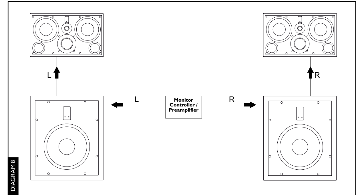
Diagram 8 – Typical Configuration – Stereo playback (Stereo Subs). A monitor controller or preamplifier output is connected to a single Input on each subwoofer. The corresponding Output of each subwoofer is connected to the Input of the main monitor on that channel. In this configuration, the Gain switch is normally set to 0dB. Note that it is also possible to connect the monitor controller output to both Left and Right channel Inputs on the subwoofer using a Y-Splitter cable. If connected in this way the "spare" output can be used to connect further subwoofers.
