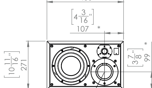
ACOUSTIC CENTRE
